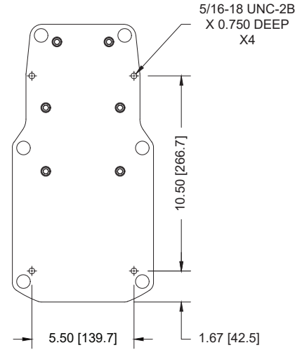
BENCH MOUNTING HOLES BOTTOM VIEW
